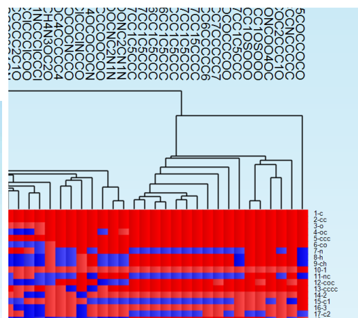
Chemoinformatics with SMILES strings - Cluster image (N-grams, zoomed)
