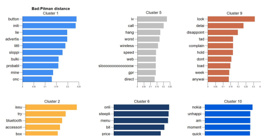
Nokia phone reviews - Bad word frequencies (bar chart)
