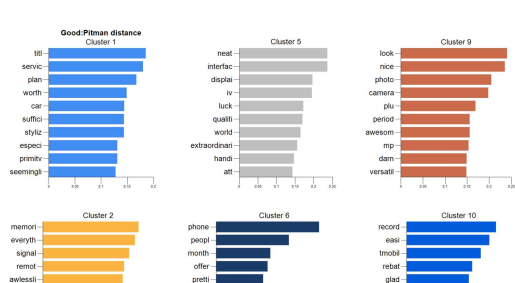
Nokia phone reviews - Good word frequencies (bar chart)
